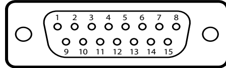
DB-15 Male
