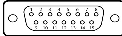
DB-15 Male
