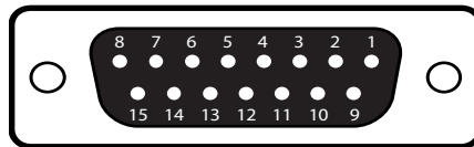
DB-15 Female
