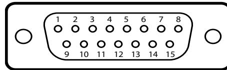
DB-15 Male
