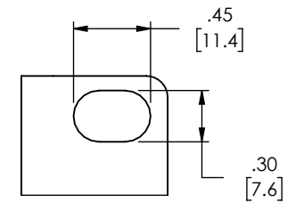
4X DETAIL A
