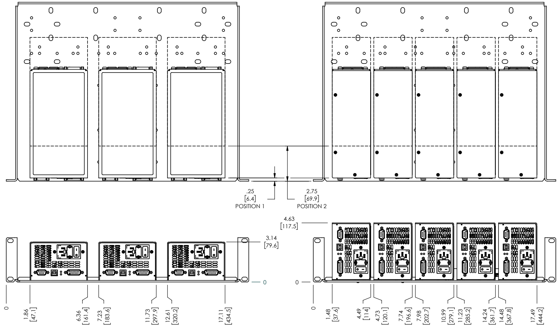
BOTTOM MOUNTING
