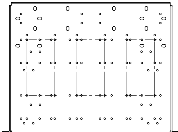
BOTTOM SURFACE MOUNTING POSITIONS
