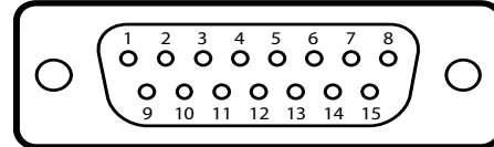
DB-15 Male
