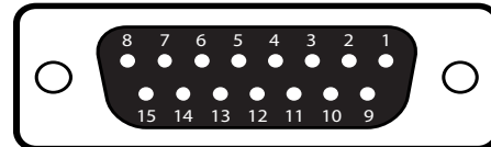
DB-15 Female
